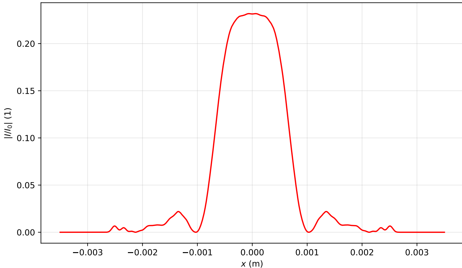
Intensity profile I(x, y = 0, z = 1.115)/I_0 , P_{in}=2.0P_{cr} , artificial time
